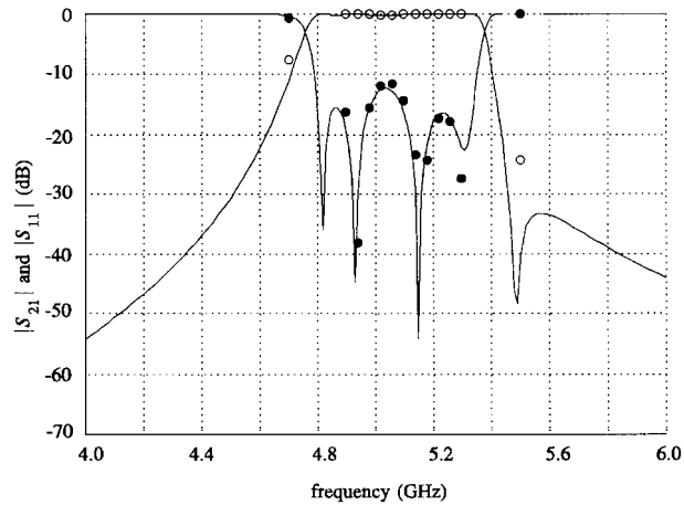
Fig. 8. The parameter extraction results. The solid lines represent the coarse model responses at \mathbf{x}_{os}^{(1)} . The circles represent the fine-model responses at \mathbf{x}_{em}^{(1)} ( \circ \circ \circ |S_{21}| , \bullet \bullet \bullet |S_{11}| ).
