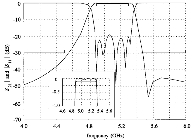
Fig. 12. Fine-model EM simulation at x_{em}^{(3)} using a fine frequency sweep.
