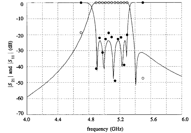
Fig. 10. The fine-model responses ( \circ \circ \circ |S_{21}| , \bullet \bullet \bullet |S_{11}| ) at \mathbf{x}_{em}^{(3)} after the second aggressive SM iteration. The solid lines represent the optimal |S_{11}| and |S_{21}| responses of the coarse model at \mathbf{x}_{os}^* .
